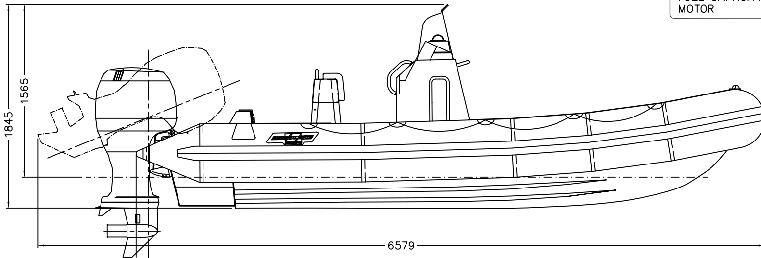
PROFILE VIEW
