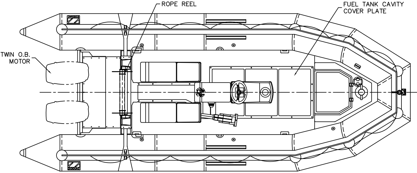
PLAN VIEW (SELF RIGHTING FRAME NOT SHOWN FOR CLARITY)
