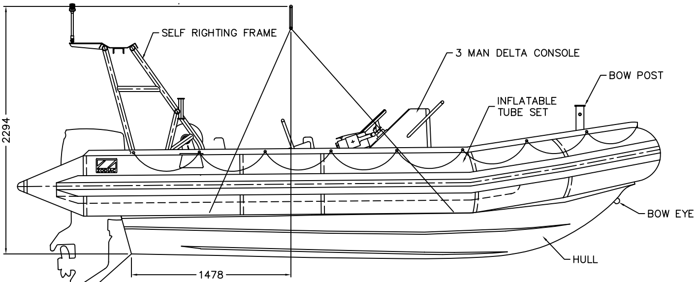
PROFILE VIEW
