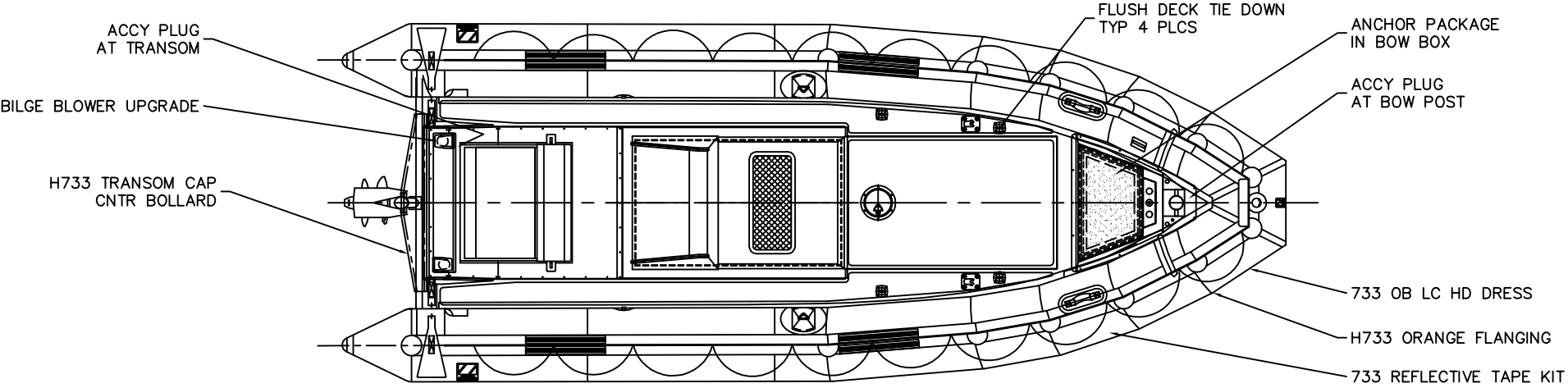
H733 IO SOLAS – PLAN DETAIL "5-D"
