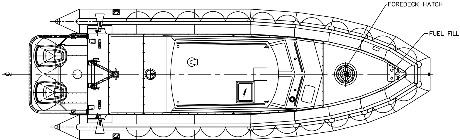
H920 OB - PLAN DETAIL "5-D"
