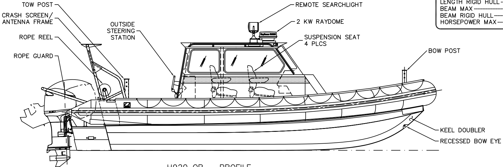
H920 OB - PROFILE DETAIL "5-A"
