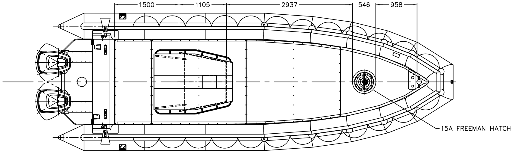
H923 OB - PLAN DETAIL "5-D"
